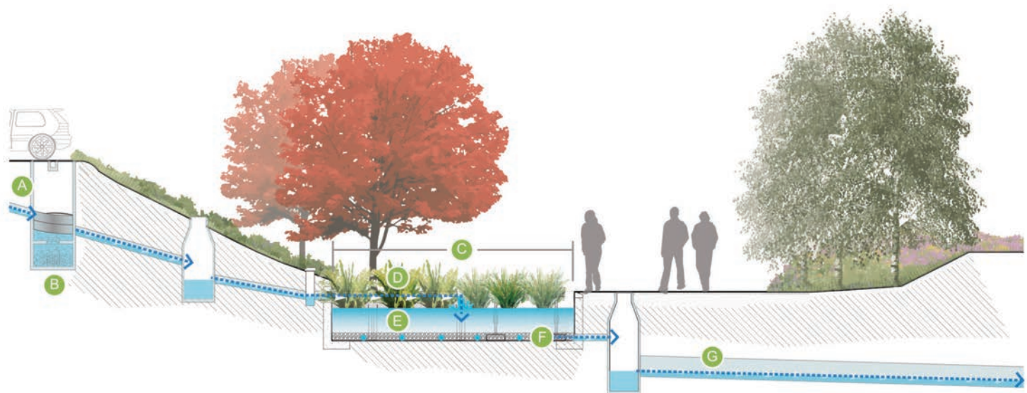
(A) untreated stormwater (B) swirl separator (C) bioretention facility (D) water tolerant plants (E) special soil media (F) underdrain to collect treated stormwater (G) clean stormwater out to city system
